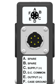
CONNECTOR OPTION
