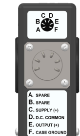
SOLDER HEADER
